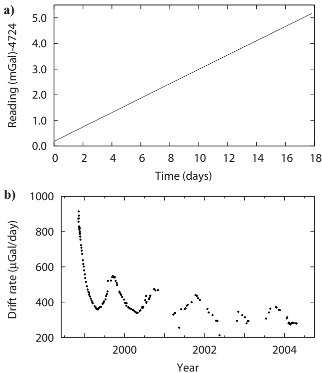
Figure 4. Linear drift characteristics of our CG-3M gravimeter. (a) Drift at a fixed, stable site over 18 days starting 24 March 2004. The linear drift rate is 280 \mu\text{Gal}/\text{day} . (b) Drift rate between November 1998 and April 2004.
