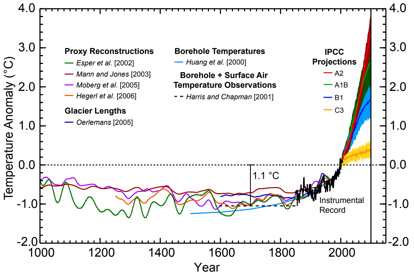
Earth's surface temperature past, present and future from Chapman, David S., and Davis, Michael G., 2010; Climate Change: Past, Present, and Future ; Eos Transactions of the American Geophysical Union , v. 91 (37), 325 – 326.
